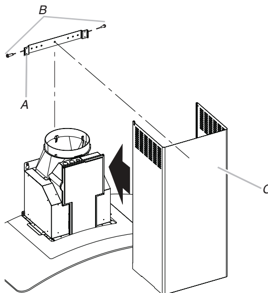
A. Bracket B. 4 x 8 mm screws C. Vent cover
